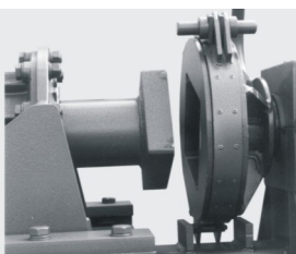
Hydraulically controlled coupling and mechanical brake (option)
